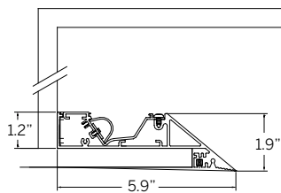
Minimal sized uplight with knife-edge detail
