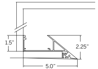
Pre-painted, non-illuminated knife edge detail
