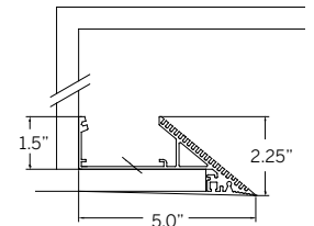
Field-Plaster and paint finished, non-illuminated
