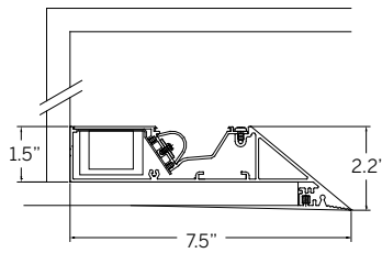
Shallow uplight with knife edge ceiling treatment
